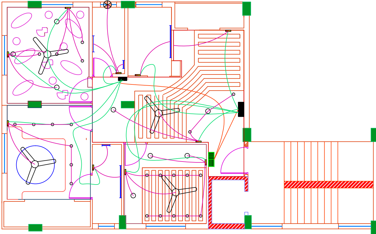
ELECTRICAL LAYOUT
